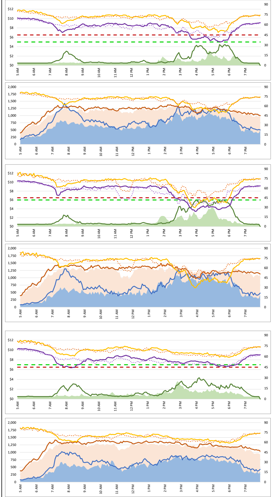
Average Speeds, Volumes & Tolls - Current (Week of 12/2 - 12/6) vs Historic (Week of 11/25 - 11/29)
