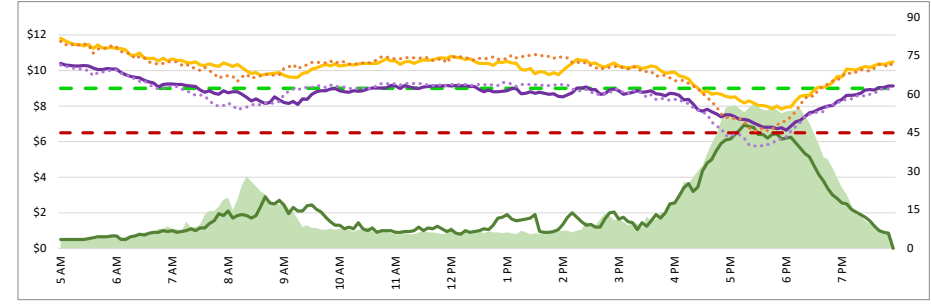
Average Speeds, Volumes & Tolls - Current (Week of 12/16 - 12/20) vs Historic (Week of 12/9 - 12/13)
