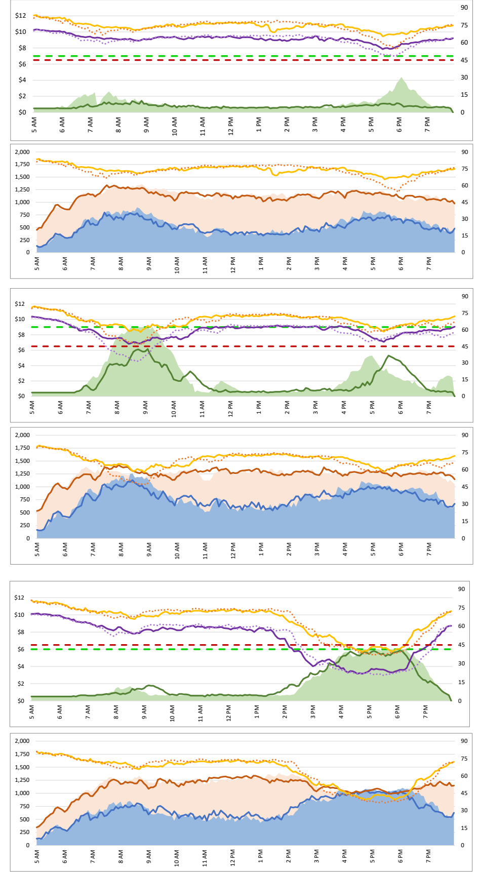
Average Speeds, Volumes & Tolls - Current (Week of 12/16 - 12/20) vs Historic (Week of 12/9 - 12/13)
